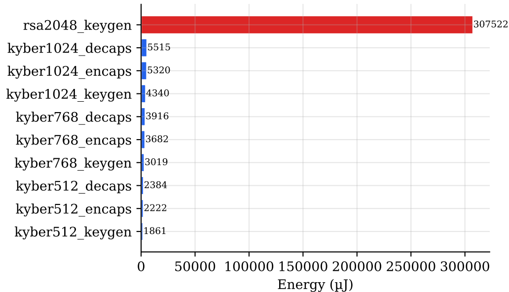
(a) STM32F446RE — INA219 Measurement (0.1 ohm shunt, 3.3V, 500 Hz)
