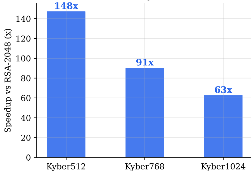
(b) Keygen Speedup vs RSA-2048 (Cortex-M4 @ 180 MHz)
