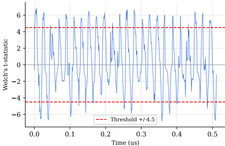
(a) Kyber512 | \max|t|=6.87 | LEAKING
