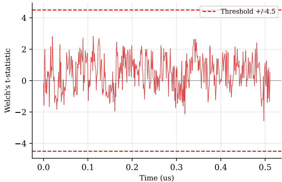
(b) RSA2048 | \max|t|=2.83 | CONSTANT-TIME
