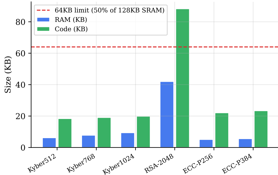
(b) Memory Footprint — STM32F446RE (128KB total SRAM)
