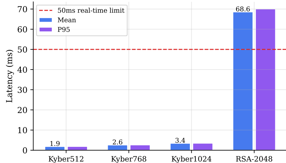
(a) Secure Channel Handshake (RPI4B loopback, 100 Mbit/s, n=100)
