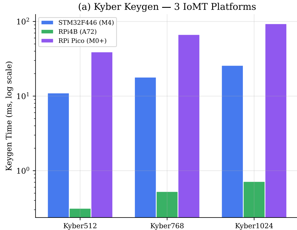
Figure 7: Cross-Platform Comparison (STM32F446 / RPi4B / RPi Pico) All platforms support Kyber512-1024 within SRAM constraints
