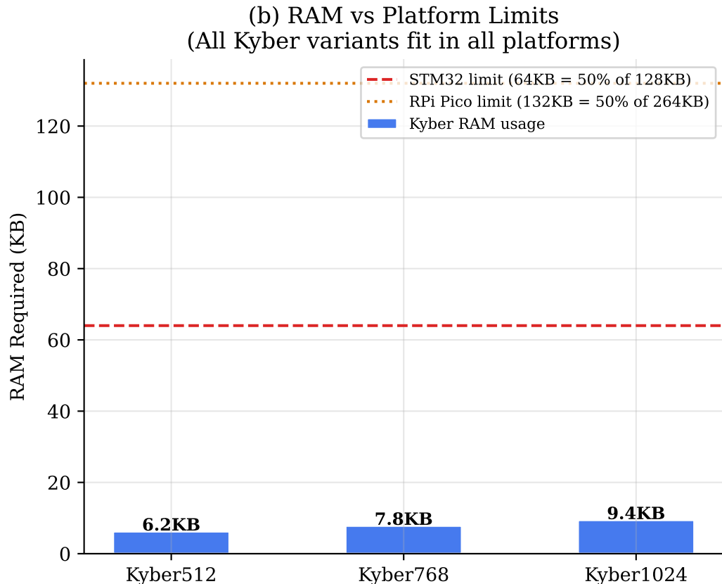
Figure 7: Cross-Platform Comparison (STM32F446 / RPi4B / RPi Pico) All platforms support Kyber512-1024 within SRAM constraints
