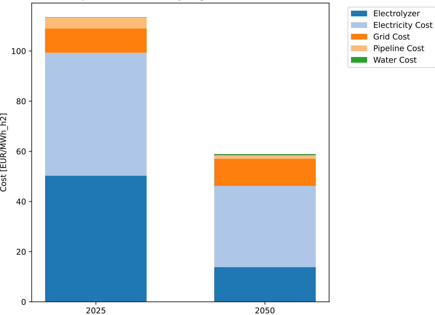
Cost Components for Green Hydrogen Production in Morocco
