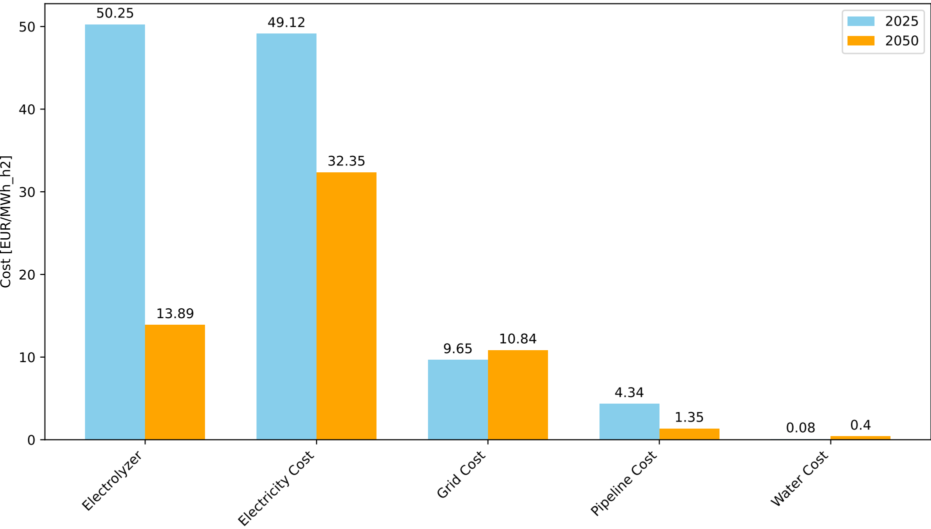
Average Cost Components for Green Hydrogen Production in Morocco
