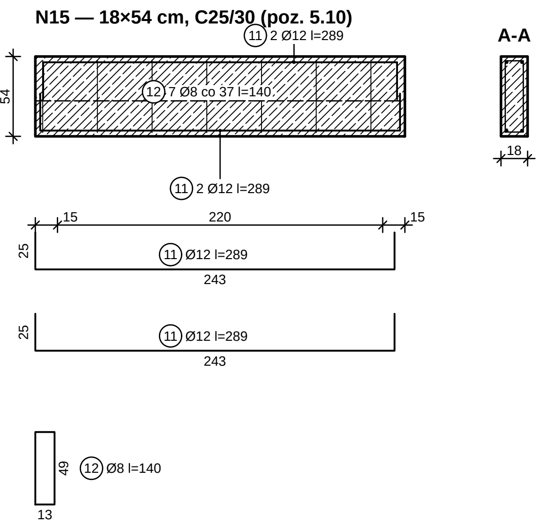
ZBROJENIE BELEK B2, B6, B7, B8, B9, B10, N15 1:25
