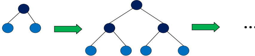
Fig. 6. Level-wise tree growth in other boosting algorithms[6].
