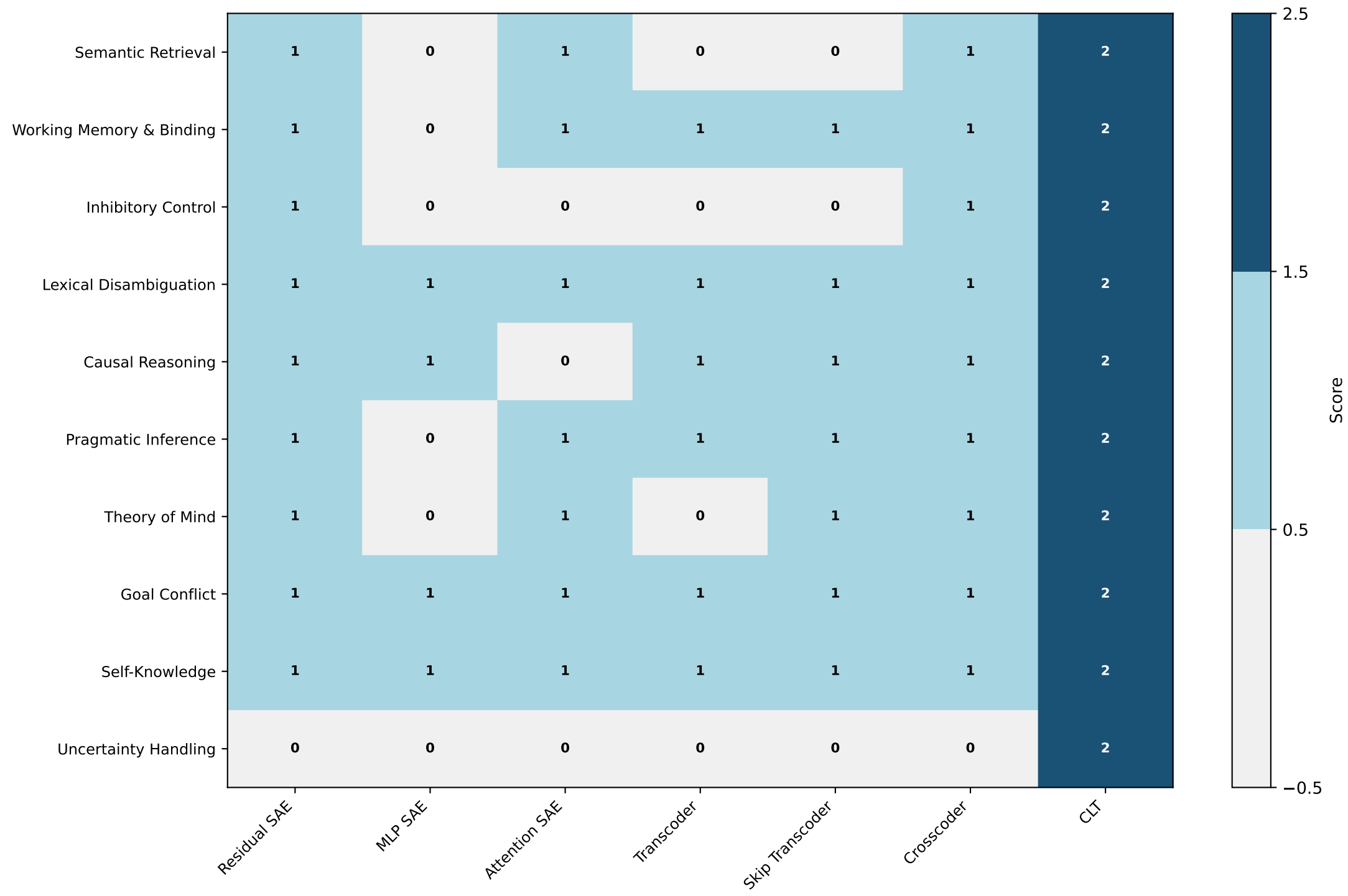
AI Anatomy: Tool x Task Coverage Grid
