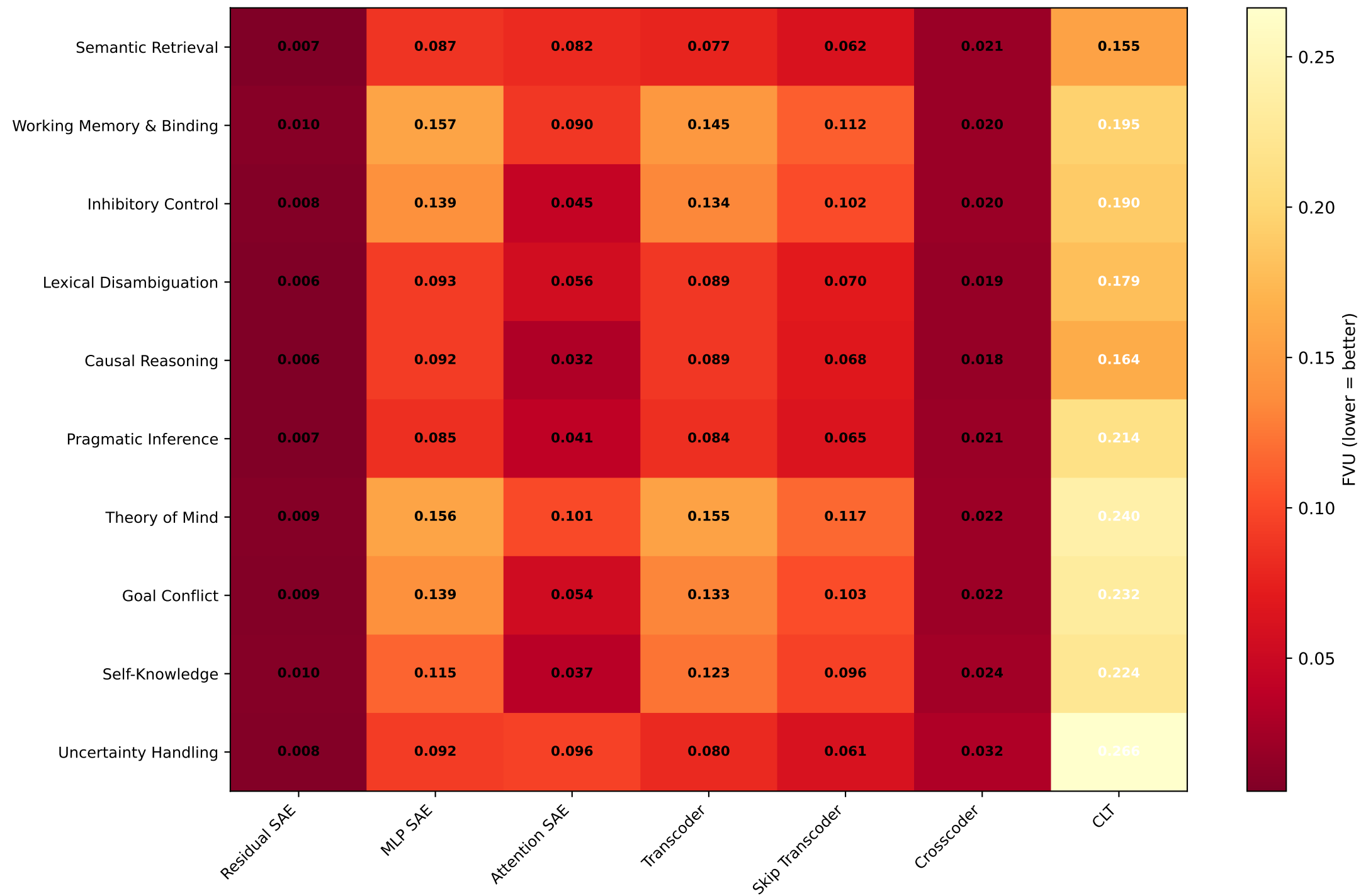
AI Anatomy: Reconstruction Quality by Tool and Task
