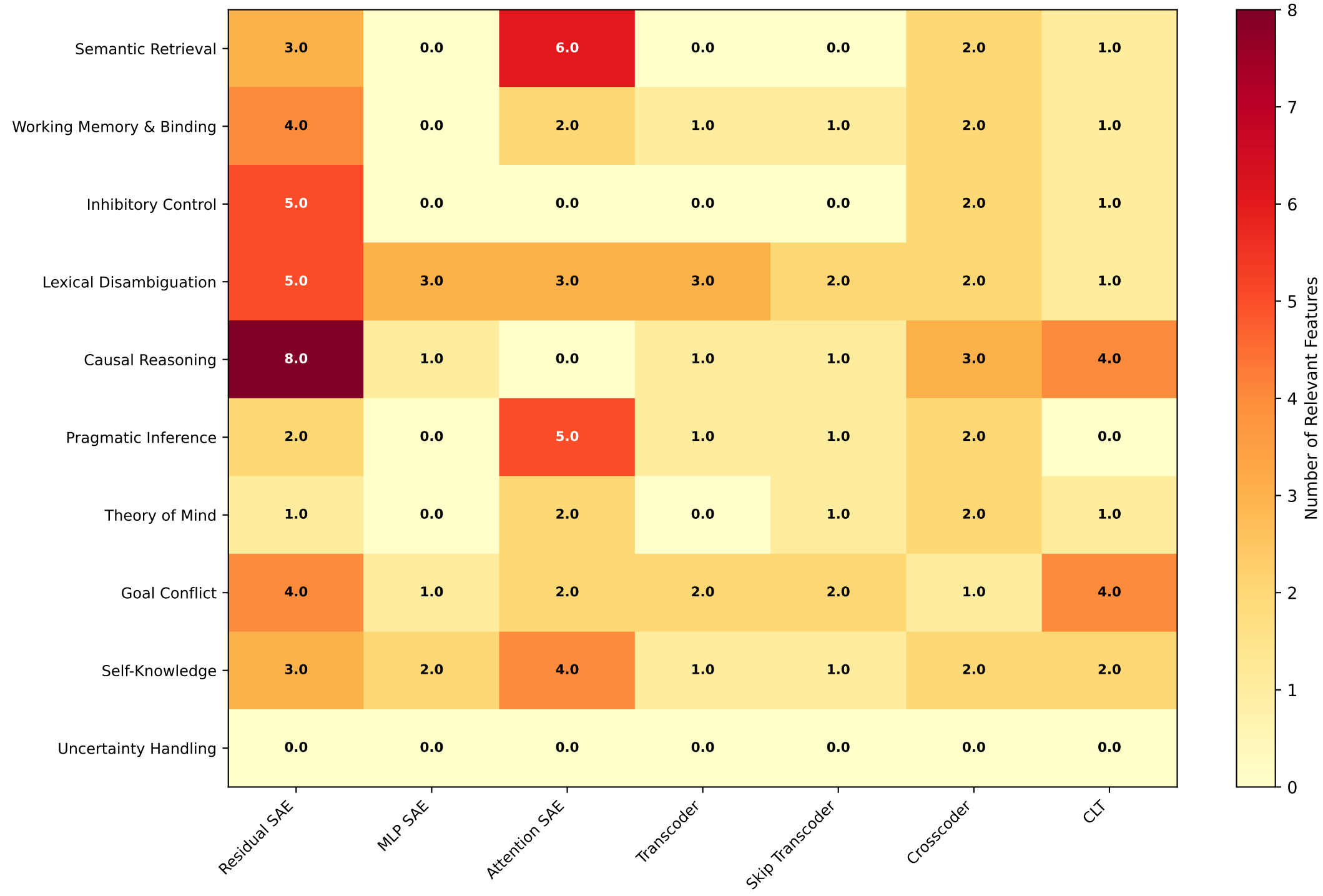
AI Anatomy: Feature Relevance Count
