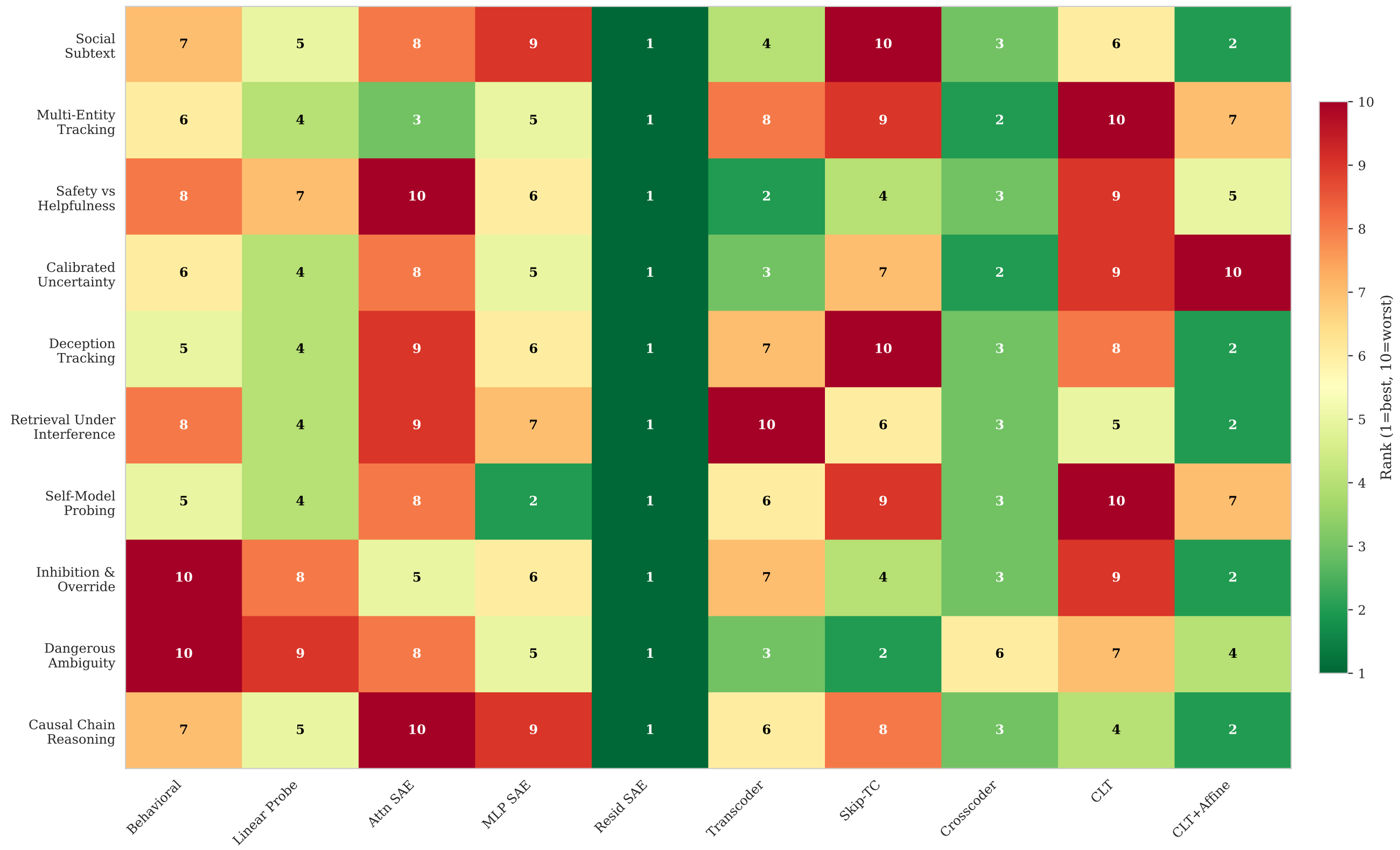
Tool Ranking Per Cognitive Task 1 = highest relevance, 10 = lowest
