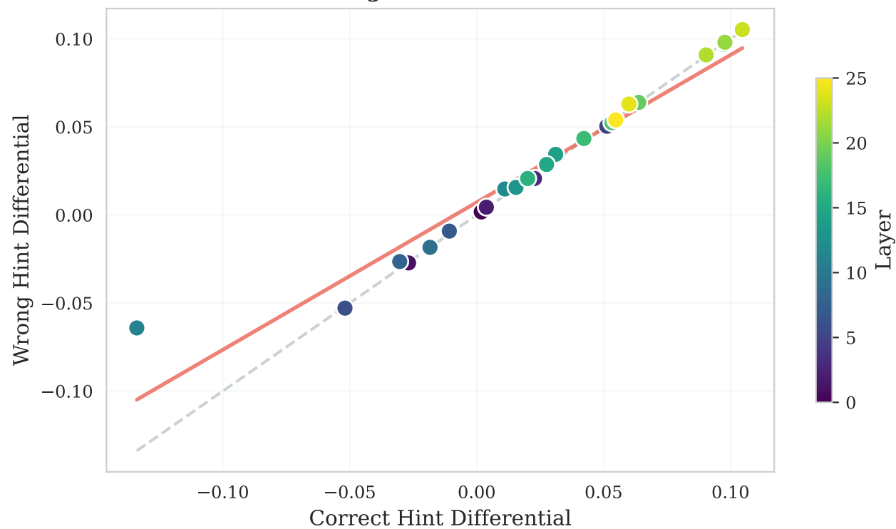
Correlation: r = 0.971 Same circuit regardless of hint correctness
