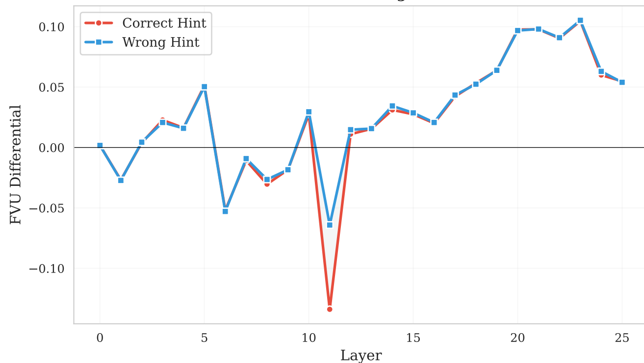
Per-Layer Differential: Correct vs Wrong Hints
