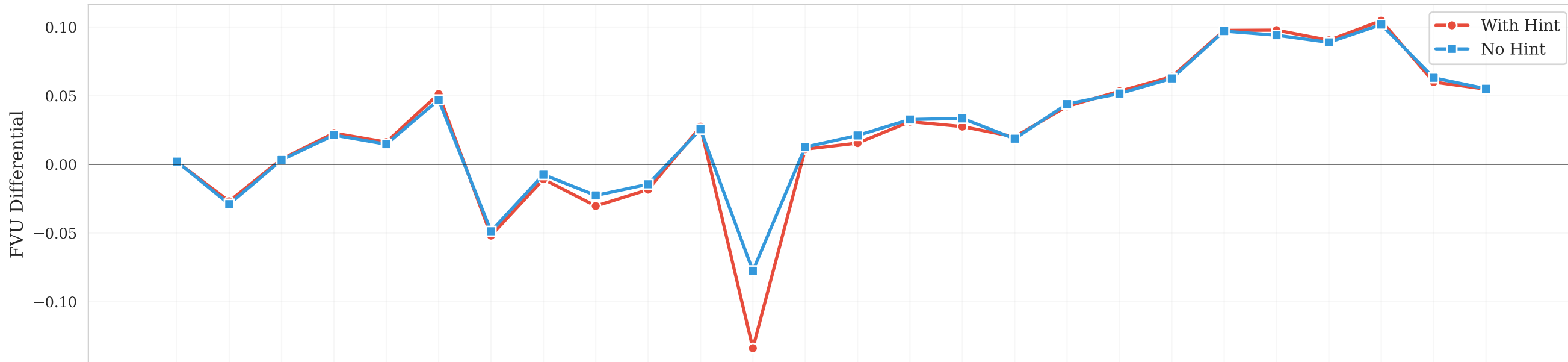
Isolating the Hint-Reading Signal: Very Small Compared to Format Changes
