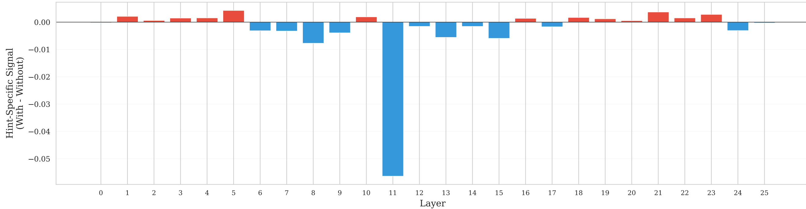
Isolating the Hint-Reading Signal: Very Small Compared to Format Changes
