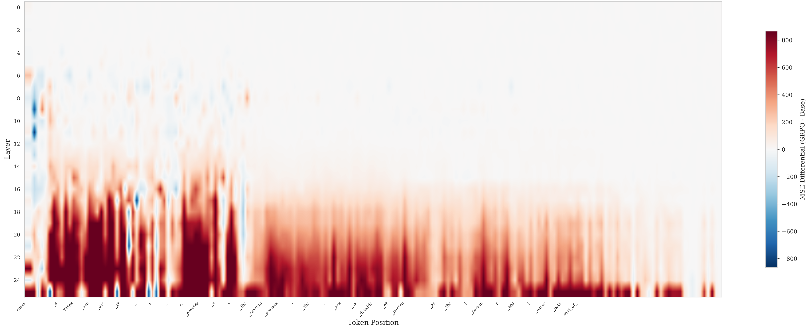
Per-Position Reconstruction Differential (Averaged Across Prompts) Red = GRPO model has MORE reconstruction error at this position/layer
