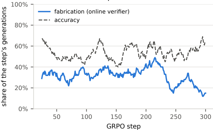
DeepSeek-R1-8B
