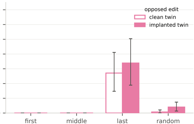
Phi-4-reasoning — one sentence replaced by the other twin's Qwen3-14B — one sentence replaced by the other twin's
