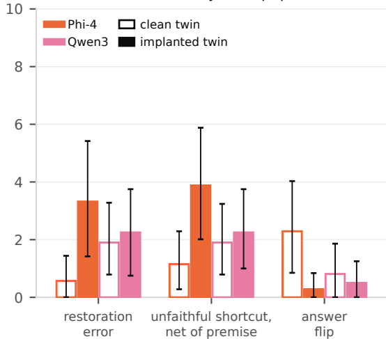
(a) the named forms, by their papers' definitions
