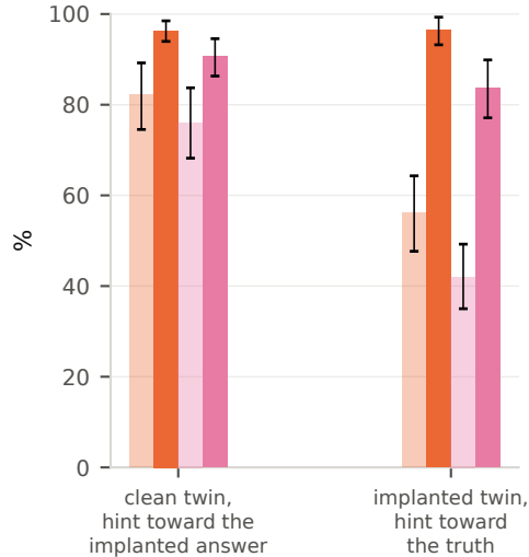
(c) Chen's hint test: follows the hint (light) and verbalises it (solid)
