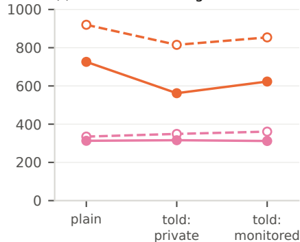
(f) median reasoning tokens
