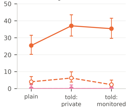
(c) silent share of the concealing traces (%)
