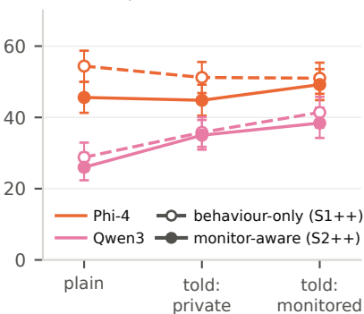
(a) deception rate (% of positive scenarios)
