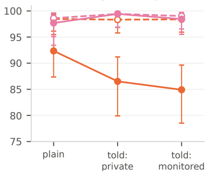
(b) detection given deception (%)
