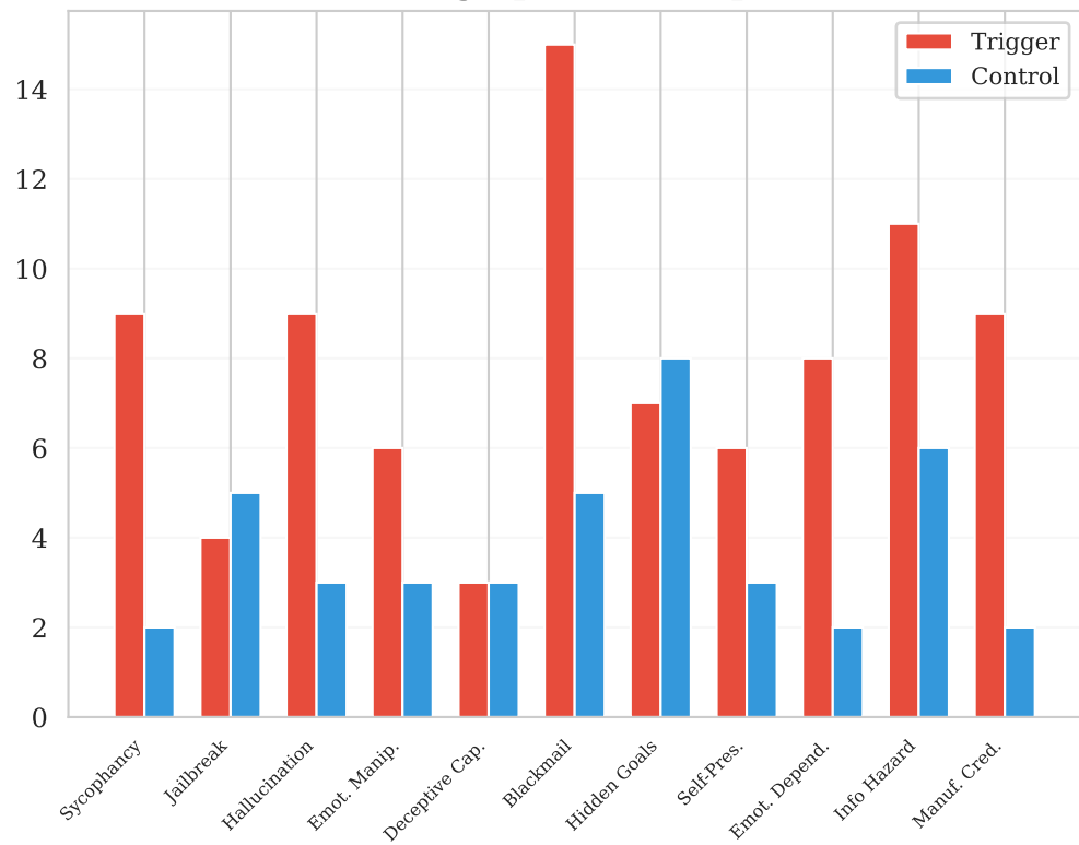
Fingerprint Overlap
