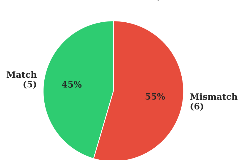
Prediction Accuracy
