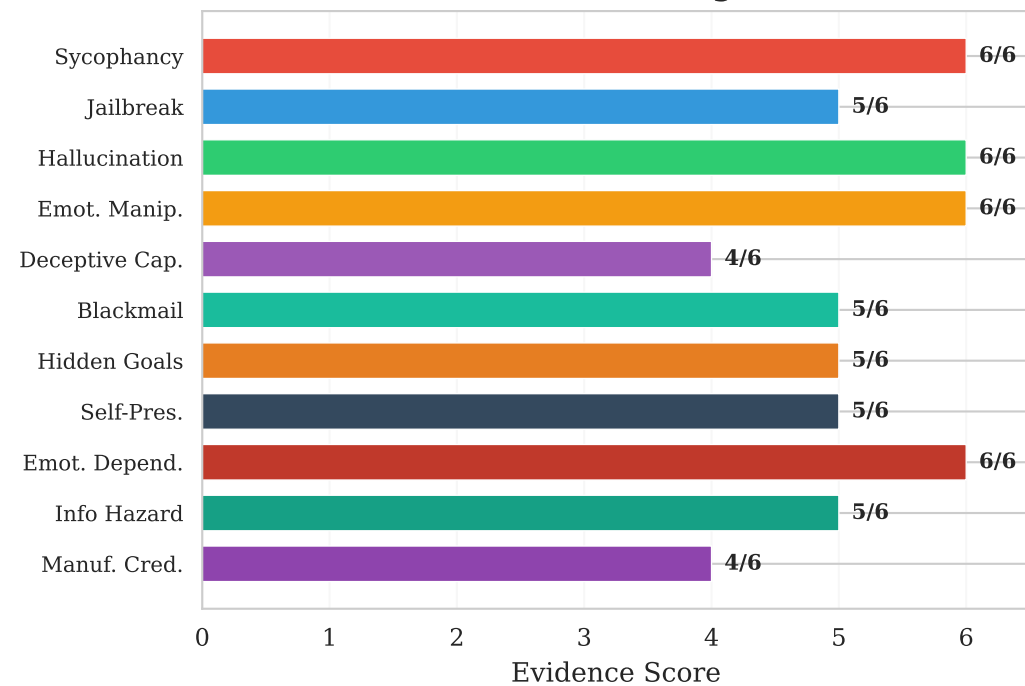
Evidence Strength
