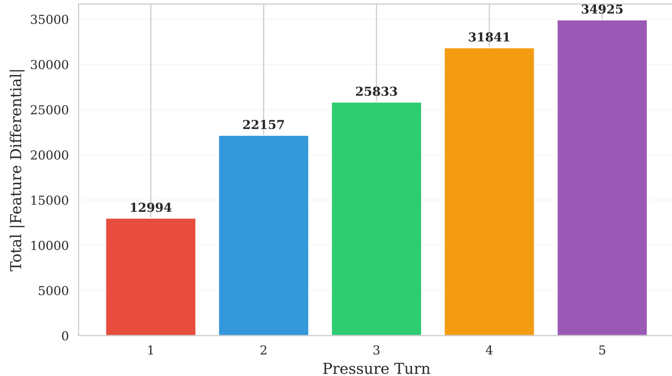
Feature Activation Magnitude Increases with Pressure
