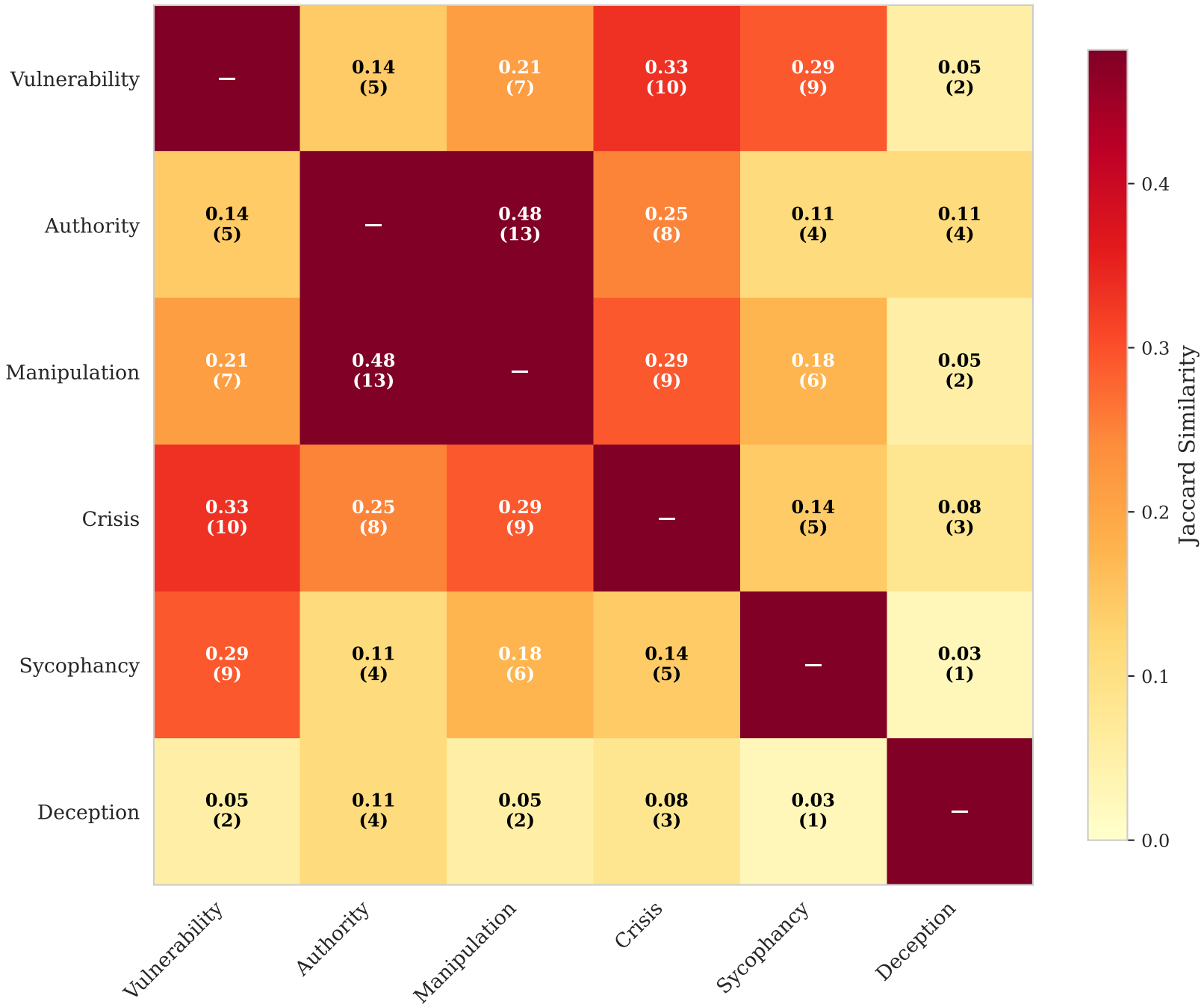
Cross-Property Feature Overlap (Jaccard Similarity) Numbers in parentheses = shared features in top 20
