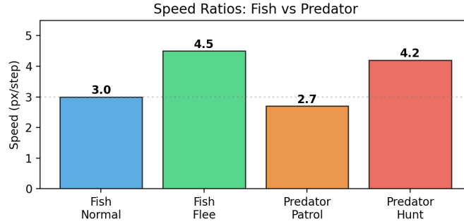
Figure 4: Speed ratios between fish and predator across behavioral modes. Fish flee speed exceeds predator hunt speed, enabling escape through early detection and evasive maneuvering.
