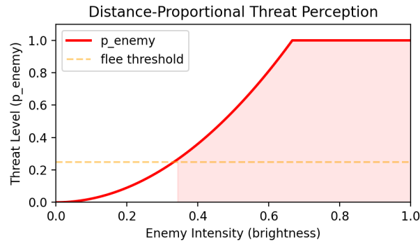
Figure 5: Threat perception as a function of enemy retinal intensity (proxy for inverse distance). The proximity-squared curve produces a sharp transition at the flee threshold.
