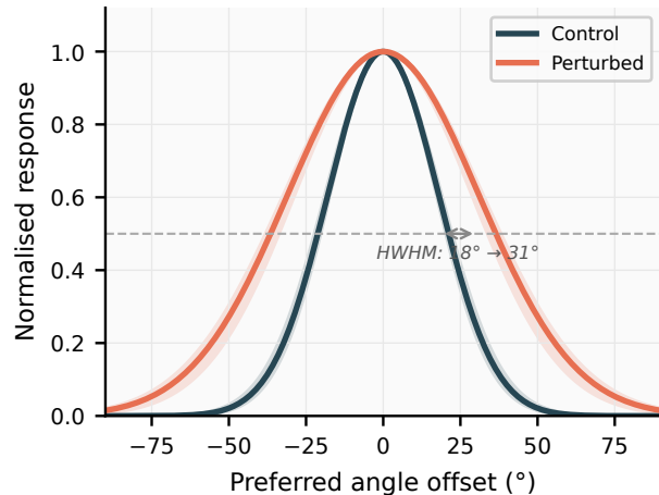
Figure 3 | Cross-level causal tracing of a precision perturbation (sensory precision weights reduced 40%; shaded = \pm 2 SE)
