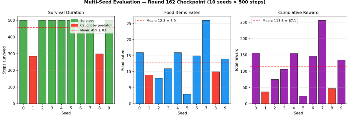
Figure 4: Multi-seed evaluation (10 seeds \times 500 steps, round 162 checkpoint). Left: survival duration ( 459 \pm 83 steps; 2/10 caught). Center: food eaten ( 12.8 \pm 5.9 ). Right: cumulative reward. Dashed red line: mean.
