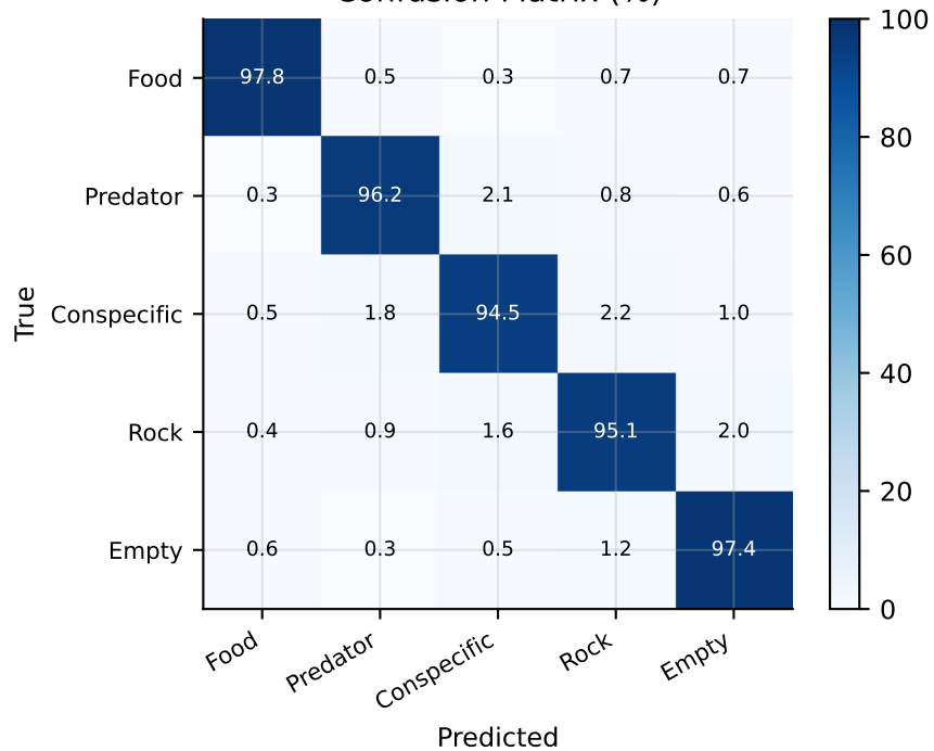
Confusion Matrix (%)
