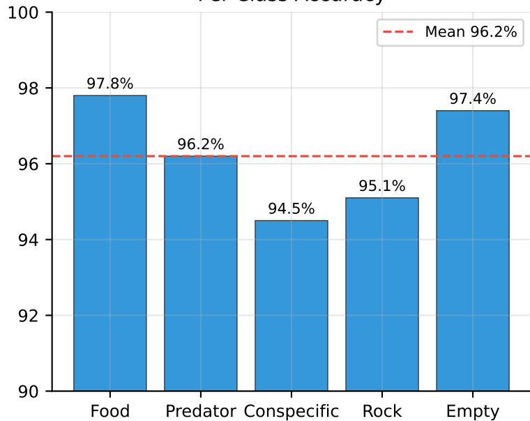
Per-Class Accuracy
