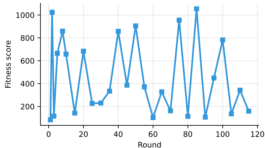
Goal Distribution
