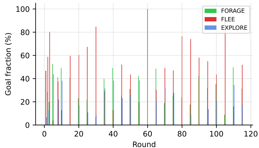
Goal Distribution
