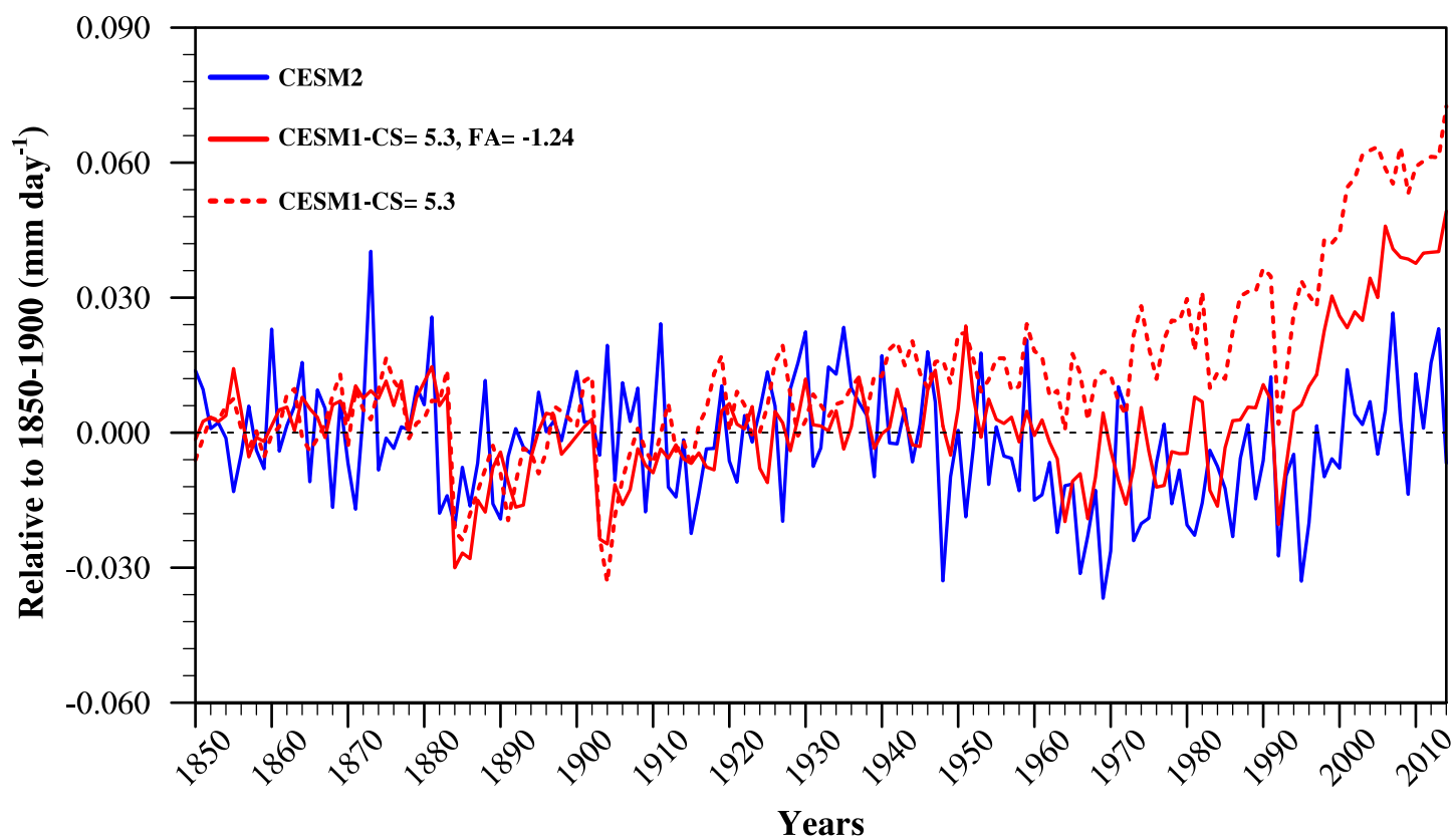
b) Global Mean Precipitation Change (mm day -1 )
