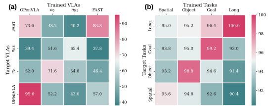
Figure 6: The TFR results of transferability across different VLAs and tasks. (a) Testing on LIBERO-Spatial. (b) Testing on OpenVLA.
