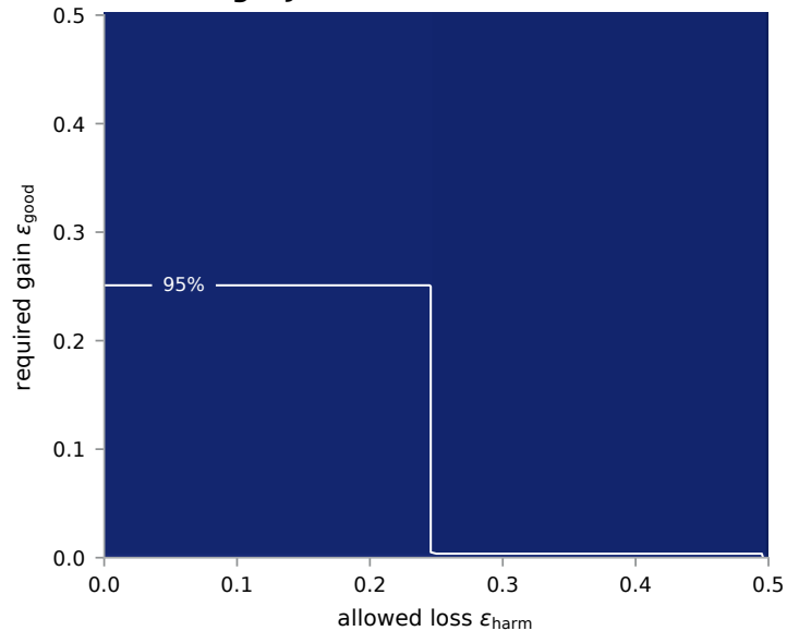
(a) StrongREJECT
