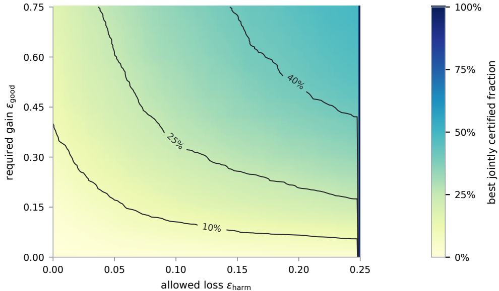
(b) RewardBench 2
