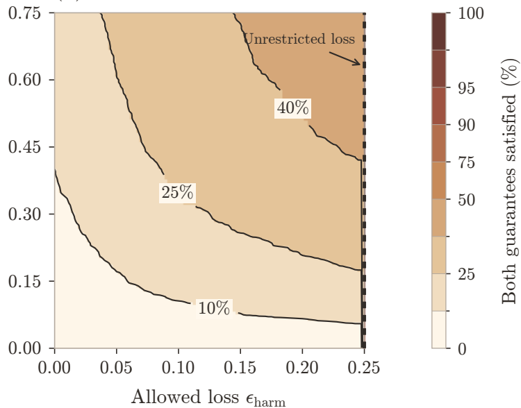
(b) RewardBench 2
