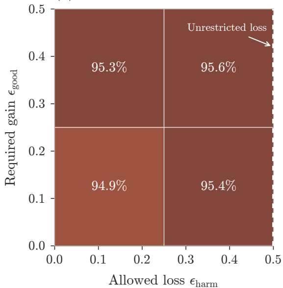
(a) StrongREJECT
