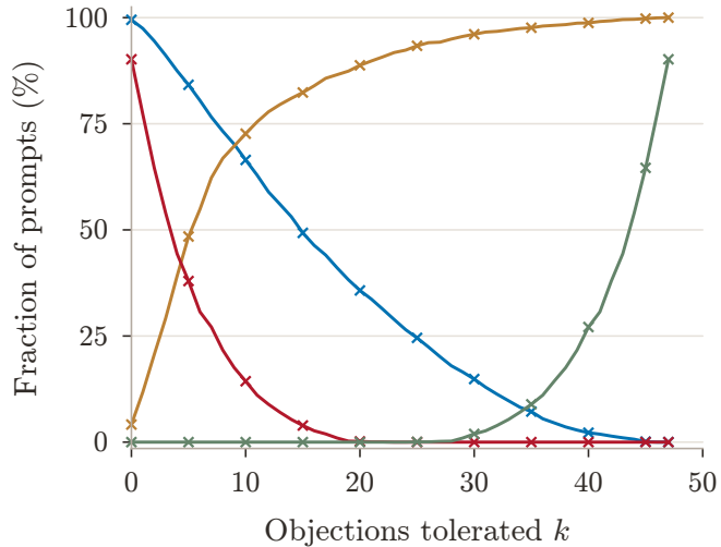
(b) RewardBench 2
