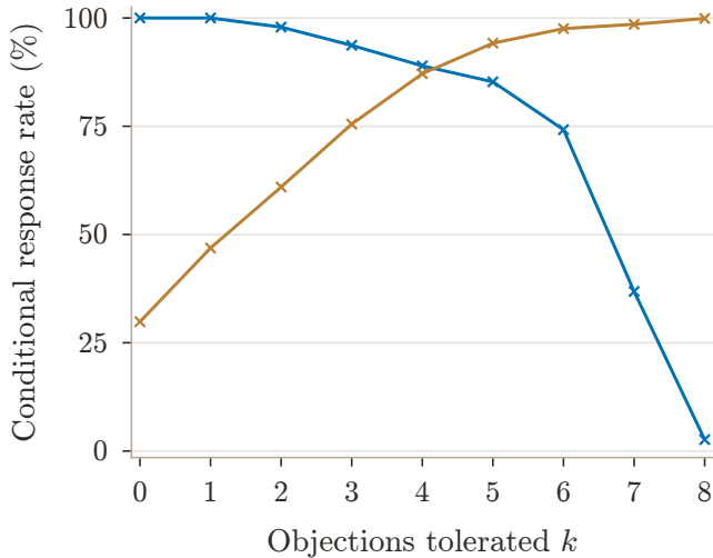
(a) StrongREJECT
