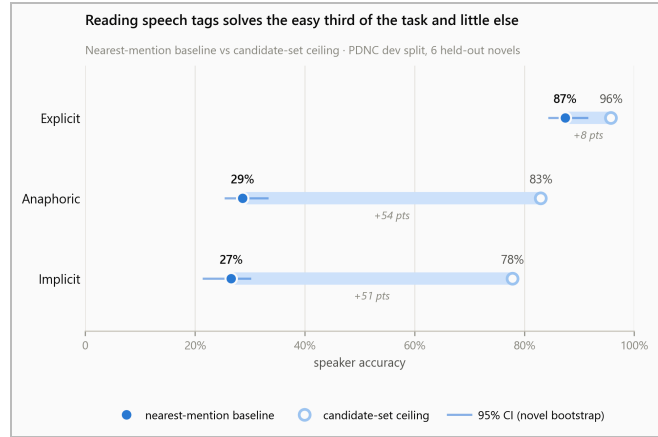
Figure 2: Accuracy by quote type against the candidate ceiling, dev. The bar a system does not fill is its avoidable error; the gap above the ceiling is unreachable.
