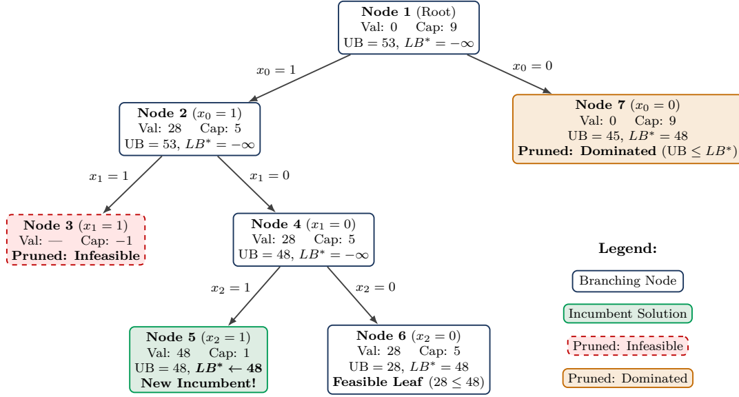
Figure 3.1: Branch and Bound search tree for the 0/1 knapsack instance (3.23) using the continuous LP relaxation. The search explores left branches first ( x_i = 1 ). When Node 5 establishes the incumbent LB^* = 48 , Node 7 on the right branch is evaluated. Its upper bound UB = 45 \leq 48 allows pruning the entire right subtree without exploring x_1 and x_2 .
