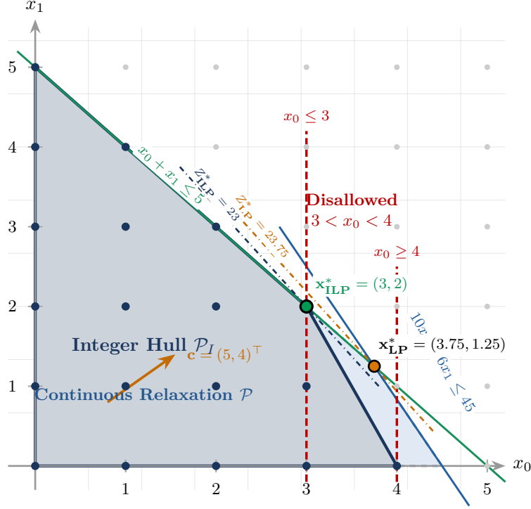
Figure 5.1: Geometric relationship between the continuous LP relaxation \mathcal{P} , the integer hull \mathcal{P}_I = \text{conv}(\mathcal{P} \cap \mathbb{Z}^2) , and LP-based branching. Discrete integer feasible solutions (navy dots) lie inside \mathcal{P} . The continuous relaxation optimum \mathbf{x}_{\text{LP}}^* = (3.75, 1.25) achieves Z_{\text{LP}}^* = 23.75 on an exterior fractional corner. Branching on x_0 creates two subproblems ( x_0 \leq 3 and x_0 \geq 4 ), carving away the non-integral strip 3 < x_0 < 4 and isolating the integer optimum \mathbf{x}_{\text{ILP}}^* = (3, 2) with Z_{\text{ILP}}^* = 23 .
