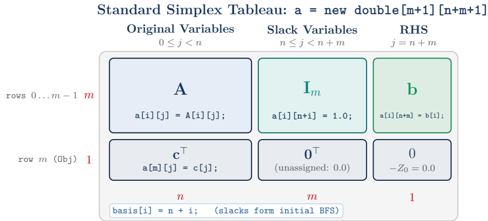
Figure 4.3: Standard Simplex tableau 2D array memory layout and Java initialization ( LinearProgramming.java ) storing m constraints and 1 objective row across n original variables, m slacks, and 1 RHS column in an array of size (m+1) \times (n+m+1) .
