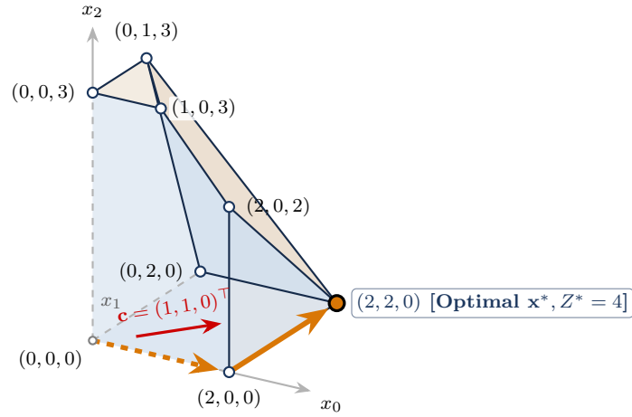
Figure 4.2: Feasible 3D polytope for Equation (4.6). The feasible region is bounded by planar facets. Vertices correspond to basic solutions where three independent planes intersect. Edges connect adjacent vertices, and Simplex walks along improving edges to reach the optimal vertex \mathbf{x}^* = (2, 2, 0) .
