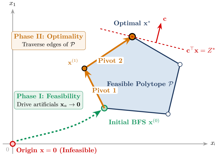
Figure 4.4: Two-Phase Simplex geometry. Phase I introduces artificial variables to create an artificial feasible space, driving them to zero along the dashed green trajectory to reach an extreme point \mathbf{x}^{(0)} of the original polytope \mathcal{P} . Phase II then traverses the edges of \mathcal{P} (solid orange path) to the optimal vertex \mathbf{x}^* .
