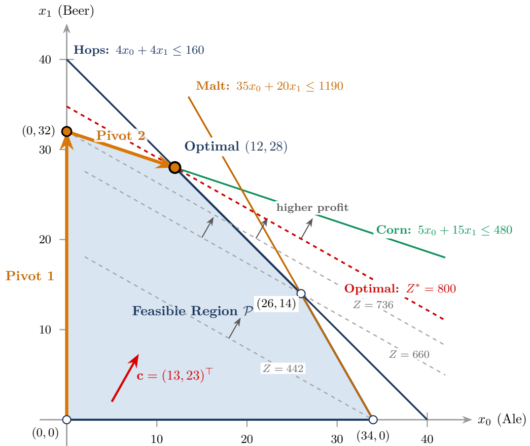
Figure 4.1: Feasible region of the Brewery Problem (Equation (4.3)). The shaded polygon \mathcal{P} is the intersection of five closed halfspaces. Dashed lines depict iso-profit contours at the extreme points ( Z = 442, 660, 736 ) up to the optimal contour ( Z^* = 800 ), with orthogonal arrows indicating the gradient direction of increasing profit. The Simplex algorithm moves from the origin (0, 0) to (0, 32) along Pivot 1, and then to the optimal vertex (12, 28) along Pivot 2.
