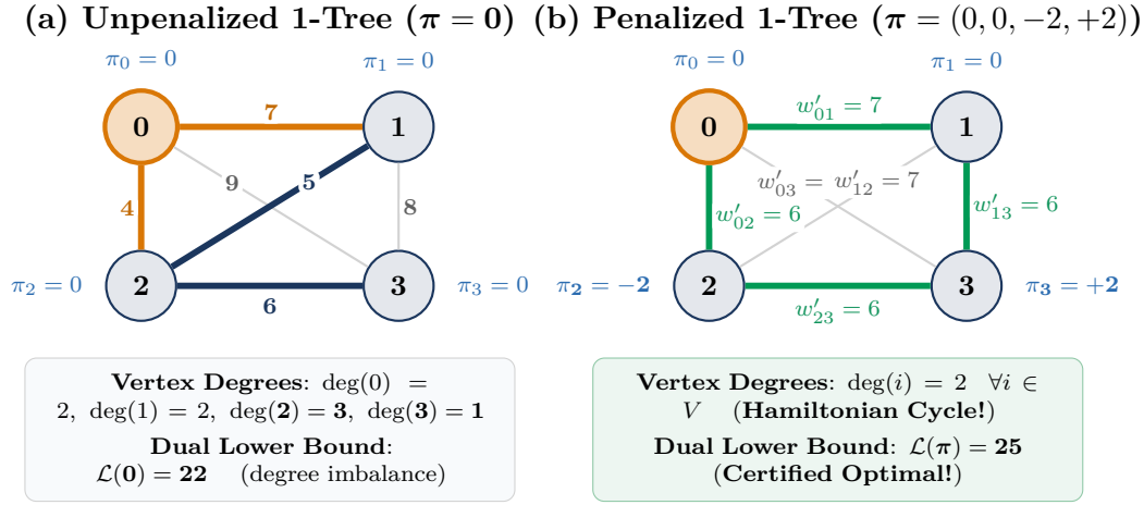
Figure 6.3: Lagrangian relaxation and multiplier transformation for a 4-vertex TSP. Panel (a): unpenalized 1-tree ( \pi = \mathbf{0} ) with degree imbalance at vertices 2 and 3 ( \mathcal{L} = 22 ). Panel (b): after introducing multipliers \pi = (0, 0, -2, +2) , the minimum 1-tree under modified weights w'_{ij} = w_{ij} - \pi_i - \pi_j becomes 2-regular, yielding a certified optimal Hamiltonian cycle of cost \mathcal{L} = 25 .
