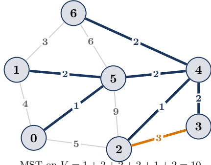
(a) MST + Cheapest Edge Relaxation (b) Minimum 1-Tree Relaxation (Root = 0)
