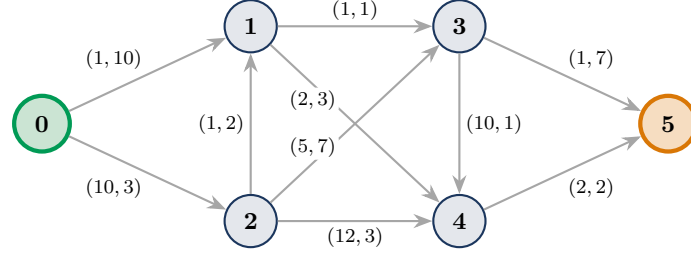
(a) Original Network: Arc Weights (c_{ij}, t_{ij}) , Budget T = 14
