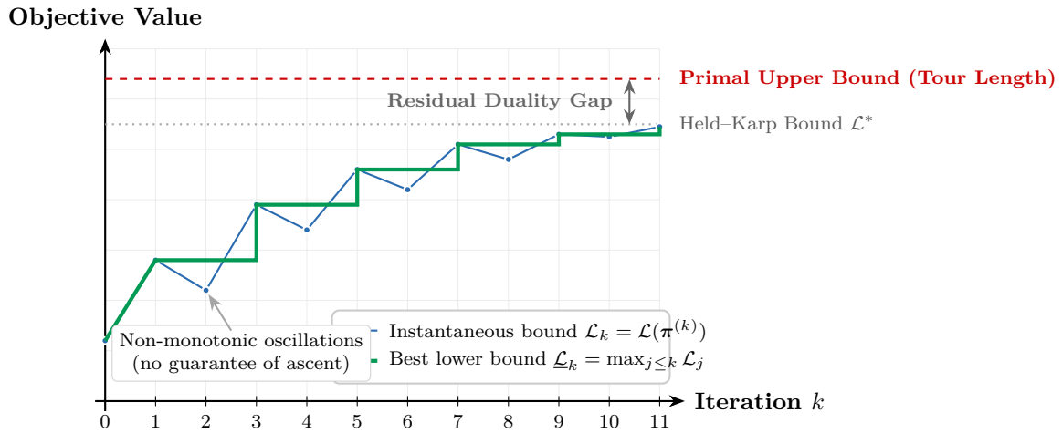
Figure 6.4: Subgradient optimization convergence for the Held–Karp TSP lower bound. The instantaneous dual value \mathcal{L}_k oscillates non-monotonically due to slope discontinuities at vertices of the 1-tree polyhedron. The running best bound \underline{\mathcal{L}}_k ascends monotonically toward \mathcal{L}^* , closing the gap against the primal upper bound.
