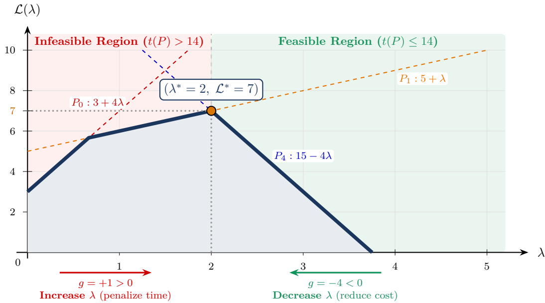
Figure 6.2: The concave piecewise-linear Lagrangian dual function \mathcal{L}(\lambda) for the RCSPP example. The optimal multiplier \lambda^* = 2 achieves the peak lower bound \mathcal{L}^* = 7 . For \lambda < 2 , the optimal path violates the budget ( t(P) > T ), yielding a positive subgradient that increases \lambda . For \lambda > 2 , the subgradient is negative, steering \lambda back toward the optimum.
