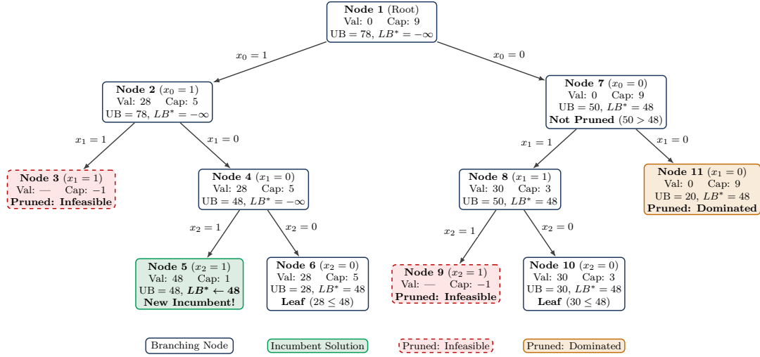
Figure 3.2: Branch and Bound search tree for instance (3.23) using the weak Capacity Relaxation. Because UB_{\text{capa}} ignores item weights, Node 7 produces an upper bound of 50 > 48 . Consequently, the branch cannot be pruned, forcing the algorithm to explore 4 additional nodes (Nodes 8, 9, 10, 11).
