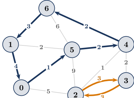
(c) Assignment (2-Factor) Relaxation
