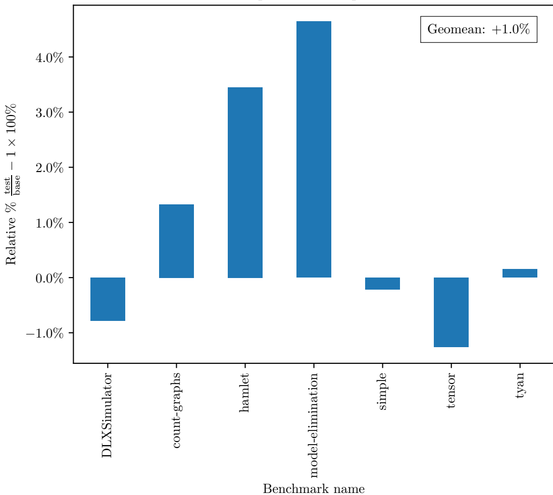
Compile time comparison
