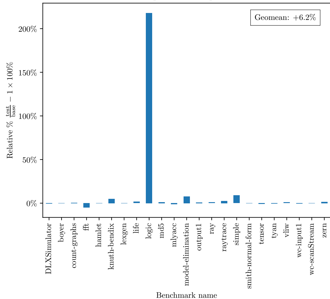
Compile time comparison
