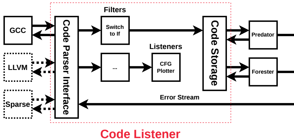
Figure 2.1: Block diagram of the legacy Code Listener infrastructure. The system is divided into interconnected modules, beginning with the code parser interface, which extracts intermediate representations from compilers such as GCC or Sparse. This data flows through optional filters, such as switch to if transformations, and listeners like the CFG plotters before being aggregated into a persistent object model within the code storage component. Finally, static analyzers such as Predator and Forester can query this code storage to perform formal verification, routing any discovered defects back through the code parser interface and the code parser’s diagnostic stream so that users and build tools receive ordinary source-located parser diagnostics [1].
