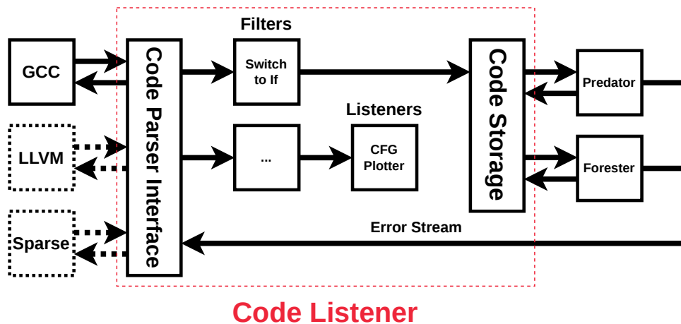
Figure 2.1: High-level architecture of the legacy Code Listener infrastructure. Reproduced from [1]
