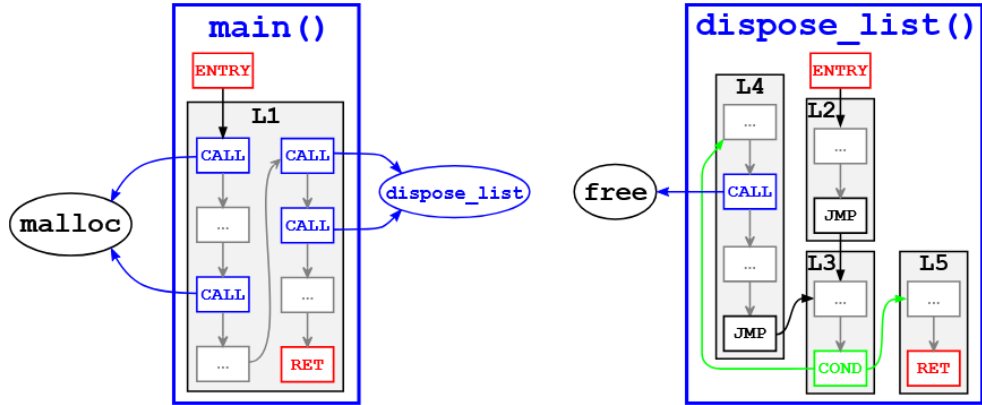
Figure 2.2: Control Flow Graph (CFG) representation of functions in the Code Listener IR. Taken from [1].
