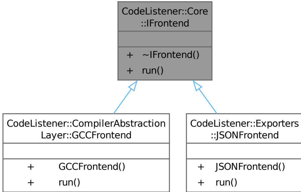
Figure 3.2: Class diagram of the IFrontend Strategy pattern [5]. The interface abstracts the source of the program model, allowing the analysis backend to operate identically whether running as a live GCC compiler plugin via GCCFrontend or as a standalone offline tool parsing JSON data via JSONFrontend .
