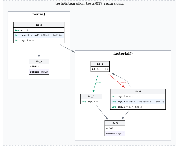
(b) COMPACT has full instruction text and operand names, ENTRY/EXIT pseudo-blocks are suppressed.
