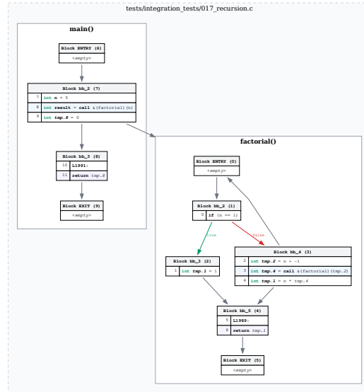
(c) FULL adds block IDs, source line numbers, and ENTRY/EXIT pseudo-blocks.
