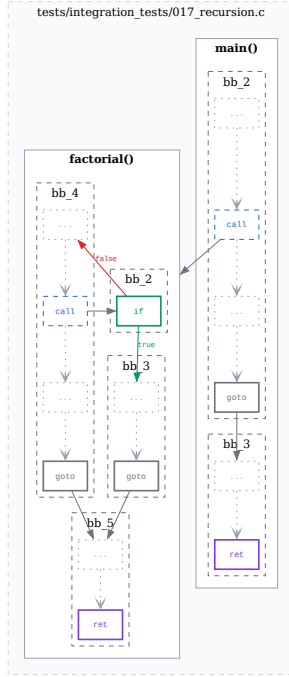
(a) CLEAN has block structure only, instruction types are shown as keywords, and mirrors the legacy look.
