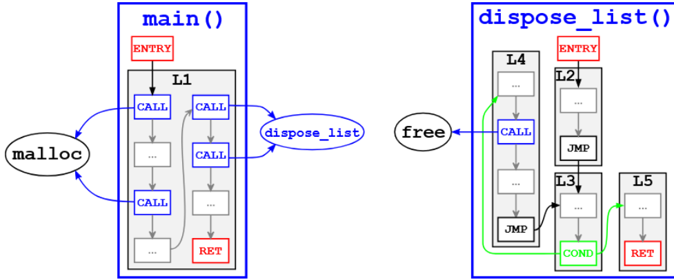
Figure 2.2: Control Flow Graph (CFG) representation of functions in the Code Listener IR. Taken from the original Code Listener paper [5].
