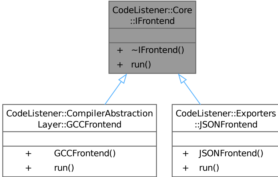
Figure 3.2: IFrontend hierarchy used by the frontend Strategy pattern [9].
