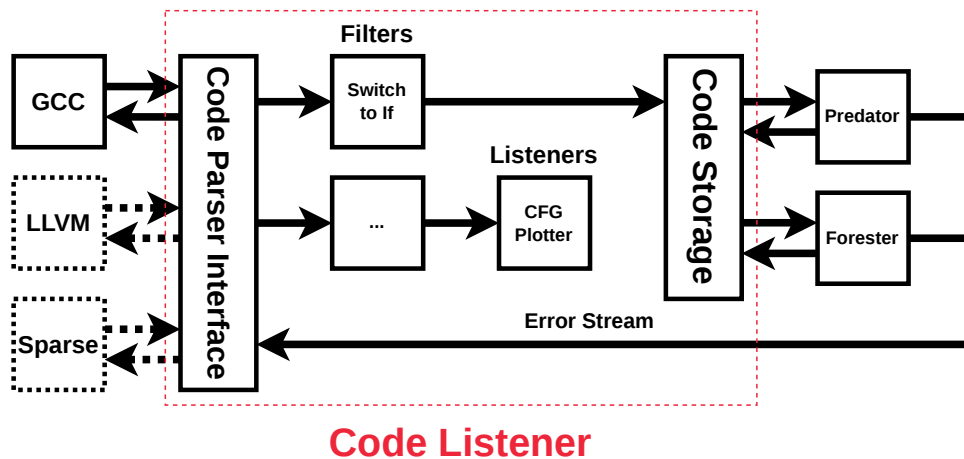
Figure 2.1: High-level architecture of the legacy Code Listener infrastructure. Reproduced from the original Code Listener paper [4]
