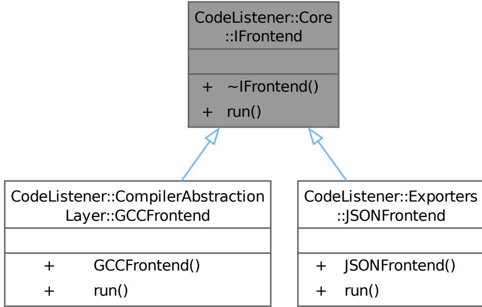
Figure 3.2: IFrontend hierarchy used by the frontend Strategy pattern [8].
