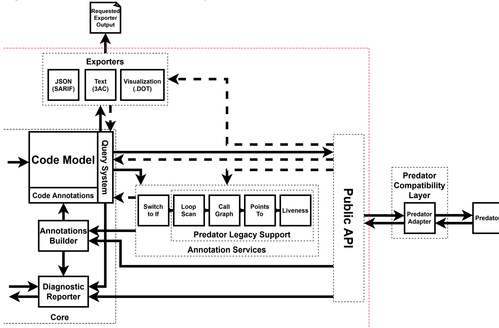
Figure 5: Detailed view of the Exporters, Annotation Services, Public API and PCL
