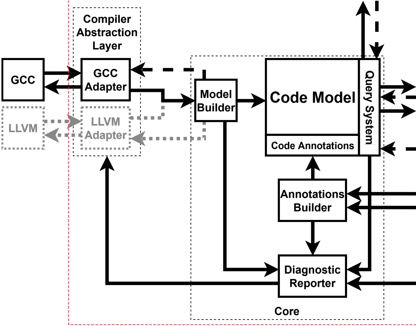
Figure 4: Detailed view of the CAL and Core
