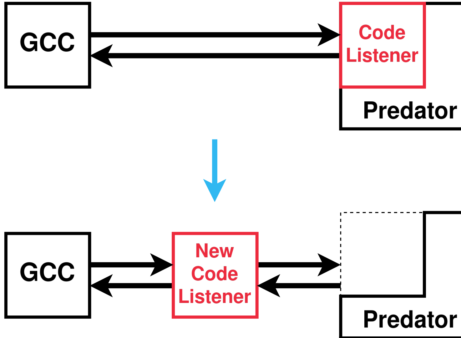
Figure 1: Decoupling Code Listener from Predator
