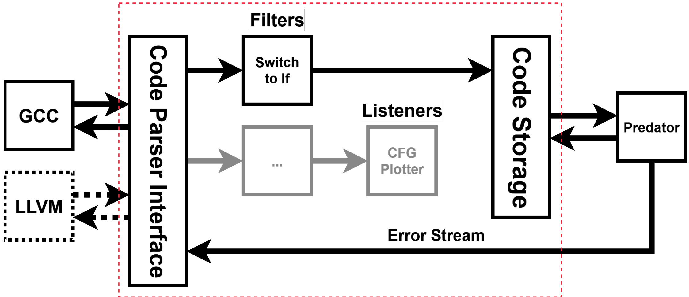
Figure 2: Current Code Listener architecture
