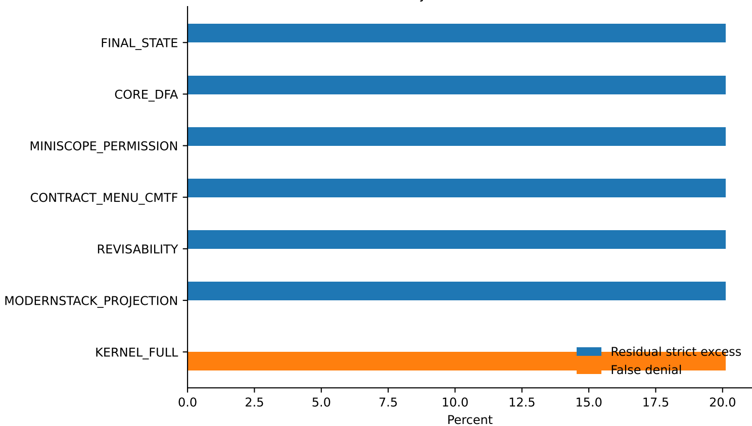
Projection baselines
