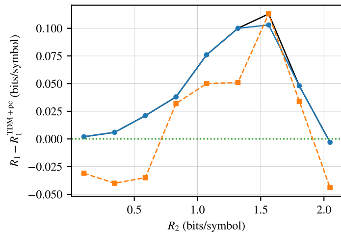
8PSK 13 / 8 dB, n = 2048
