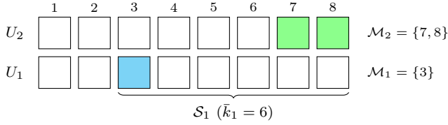
Fig. 3. Algorithm 2 for n = 8 , k_2 = 2 , \bar{k}_1 = 6 , and k_1 = 1 . The 5G NR order from least to most reliable is (1, 2, 3, 5, 4, 6, 7, 8), so \mathcal{M}_2 is its last two entries and \mathcal{M}_1 is the least reliable entry of S_1 = \{3, \dots, 8\} .
