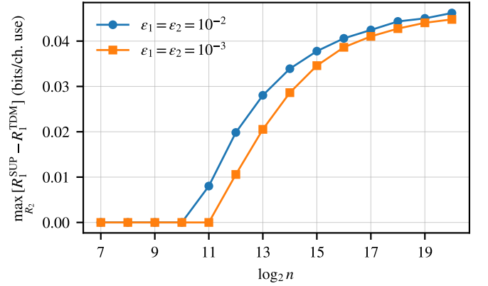
Fig. 5. Largest advantage in R_1 of \mathcal{R}^{\text{SUP}} over \mathcal{R}^{\text{TDM}} at equal R_2 , for BSBC(0.01, 0.10). A value of 0 means that the SUP region lies inside the TDM region.
