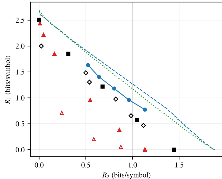
8PSK, 13 / 8 dB, n = 128
