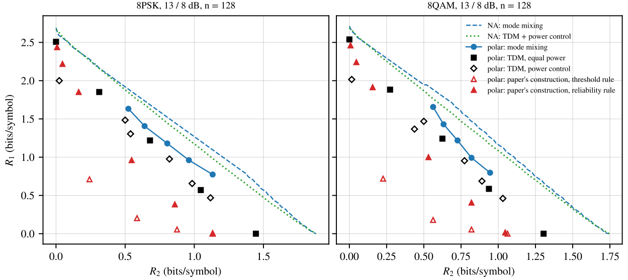
Figure 5: Polar codes at n = 128 (markers; SC decoding, per-user block error rate \leq 10^{-2} ) against the normal approximations at the same blocklength (lines), hard-decision 8PSK and 8QAM at 13/8 dB.
