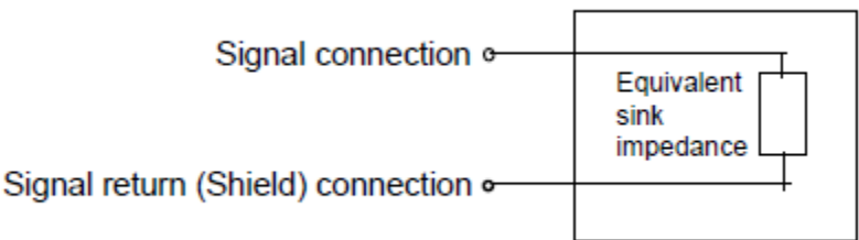
FIGURE 13b. Equivalent circuit of HB interface when receiving a Type A signal
