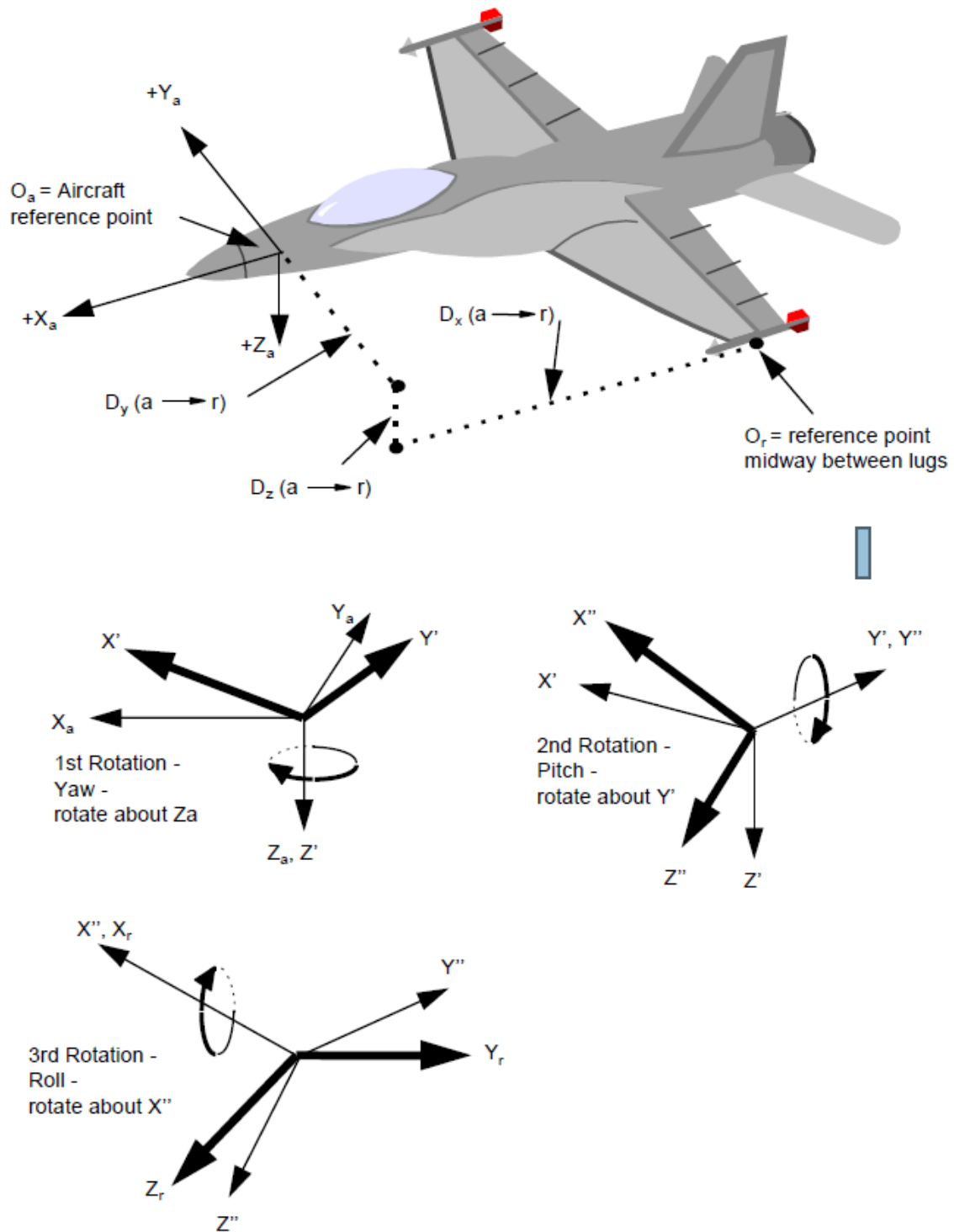
FIGURE B-6. Aircraft-store alignment
